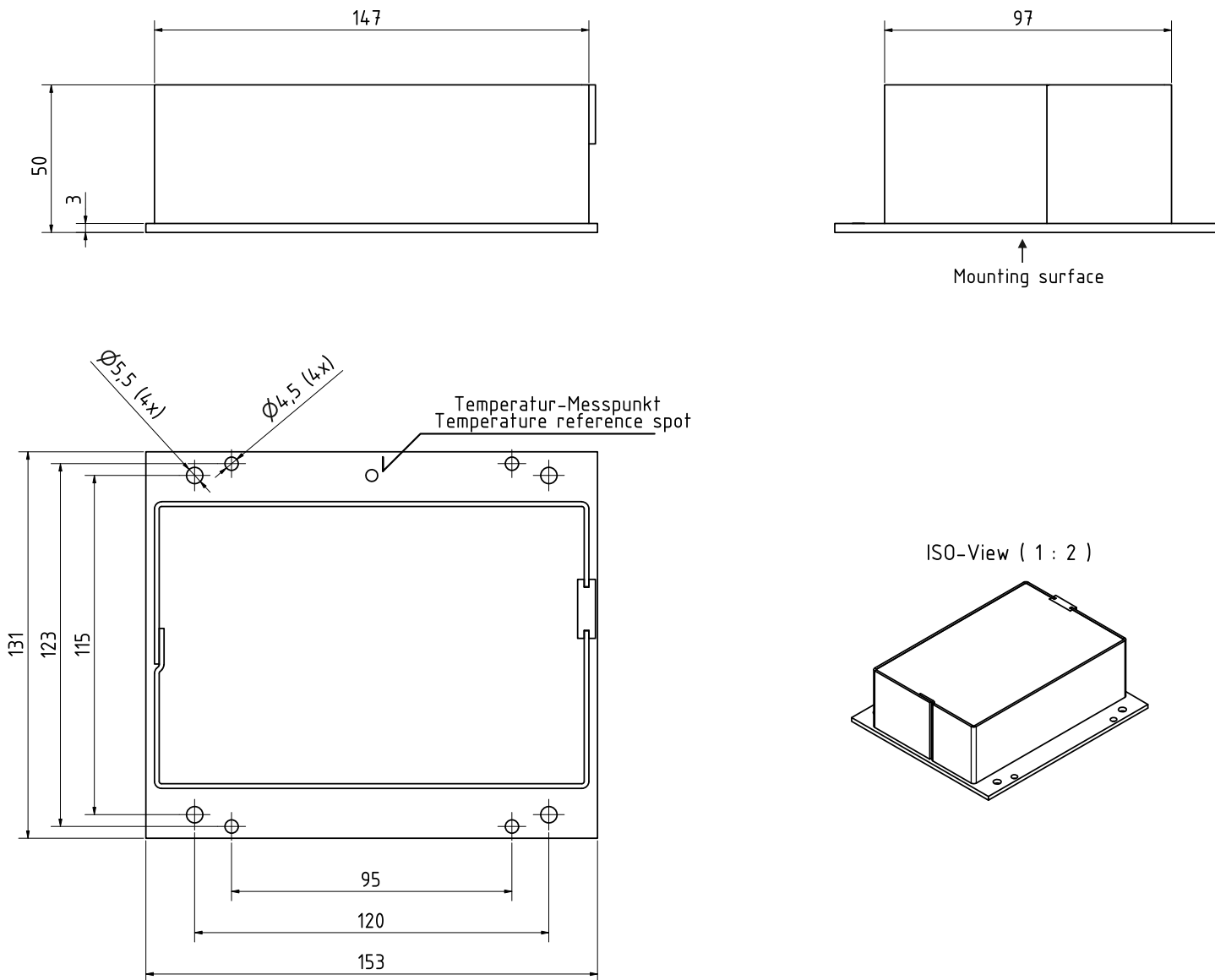
Figure 8.1: Dimensions
