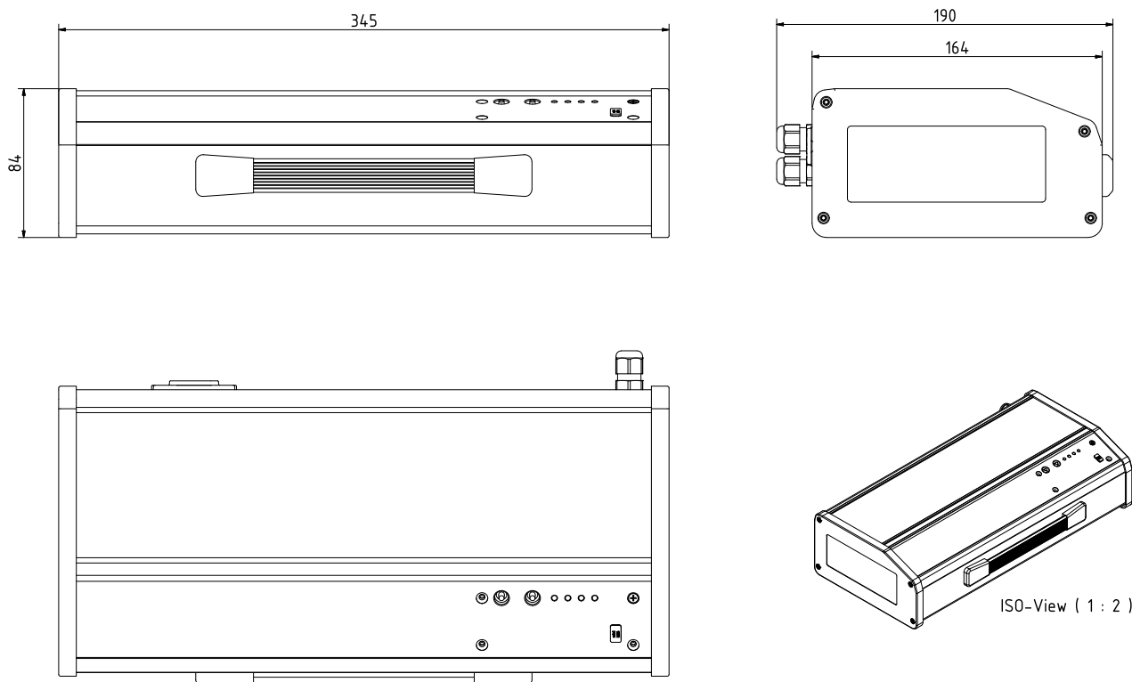
Figure 7.1: Dimensions
