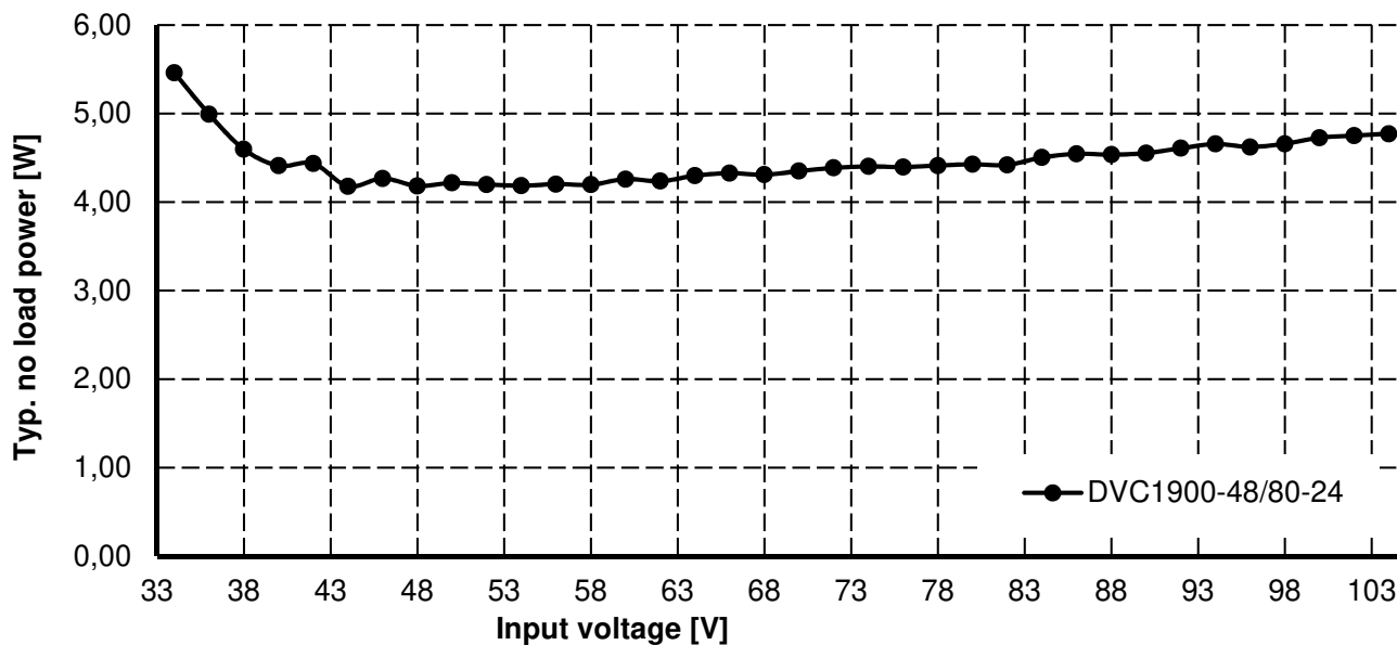
Figure 8.1: No-load power
