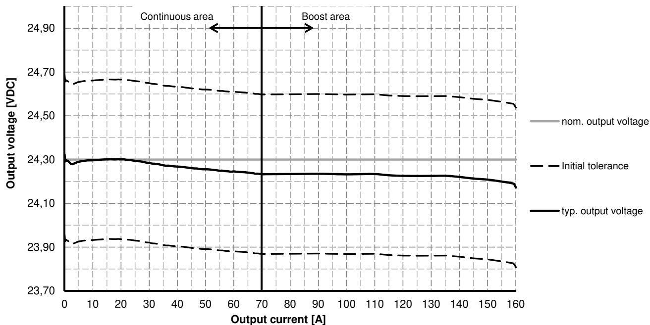
Figure 8.7: Typ. output voltage and initial tolerance
