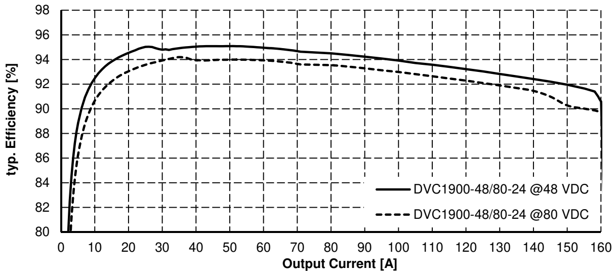
Figure 8.4: Efficiency depending on the output current
