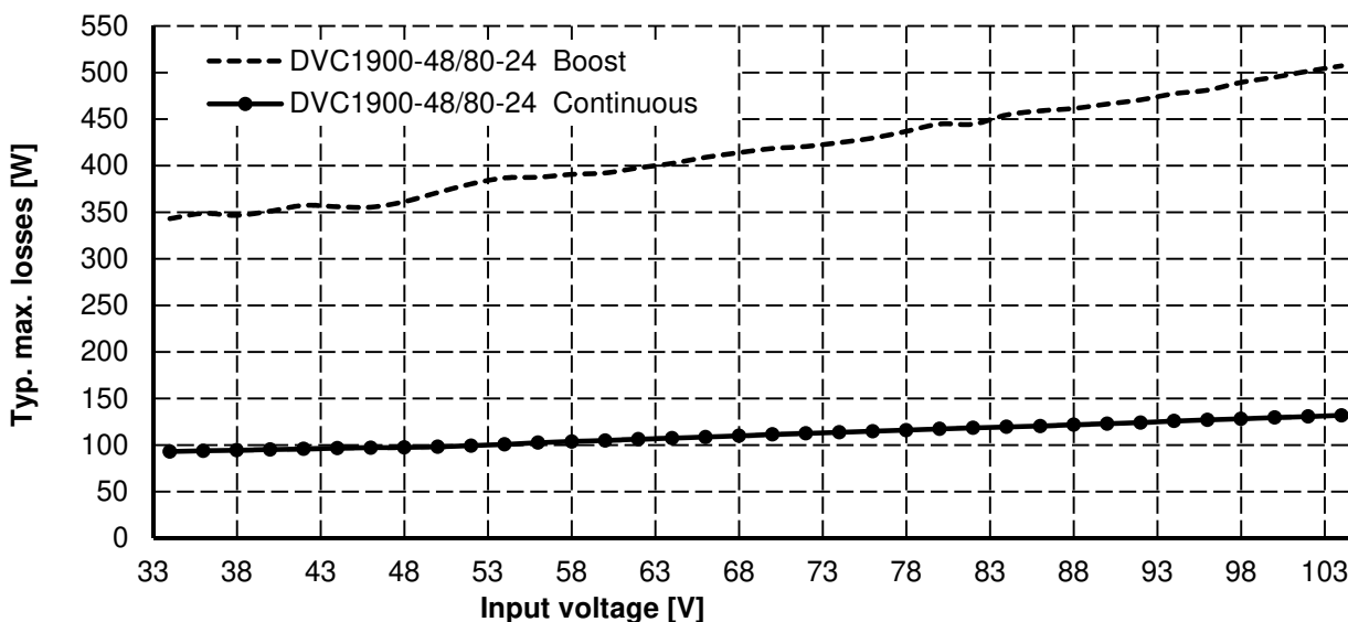
Figure 8.6: Typ. maximum power loss
